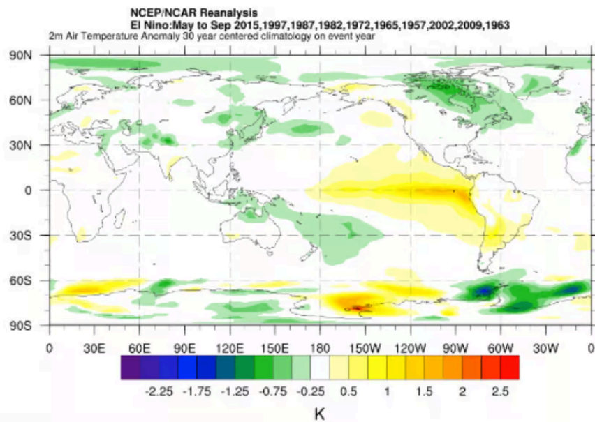
Figure 1: Air temperature anomalies during El Niño (Summer)
