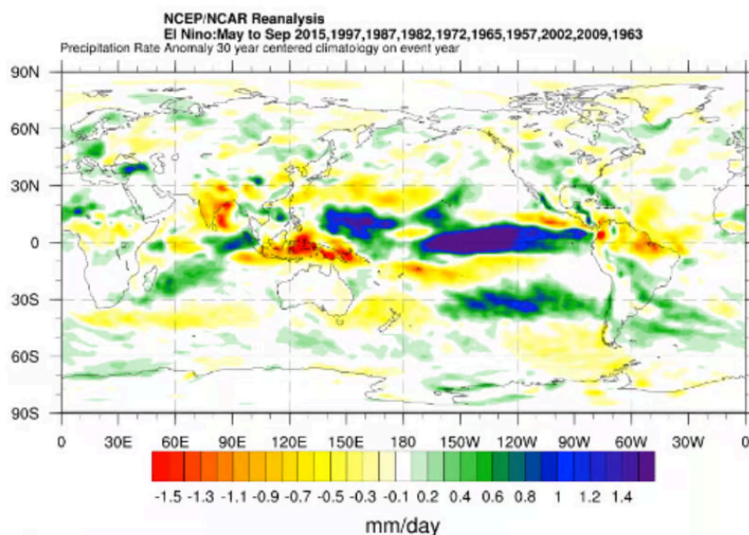
Figure 2: Precipitation rate anomalies during El Niño (Summer)
